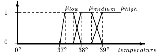
Fig. 4. Fuzzy sets representing the concept fever .
