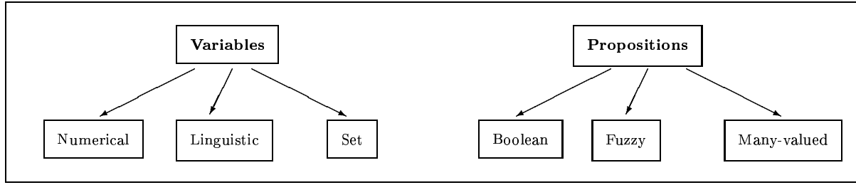
Fig. 2. Types of variables and propositions.
