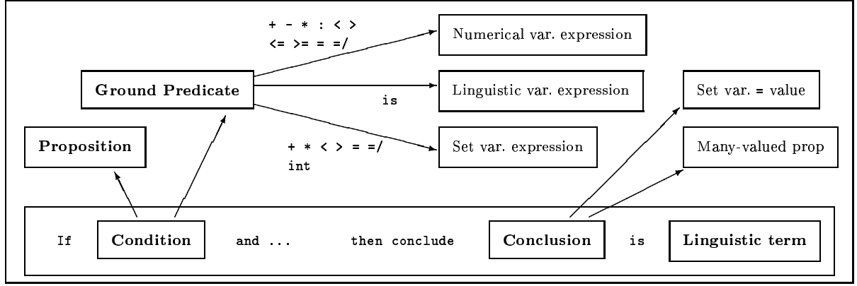
Fig. 5. Rule structure.
