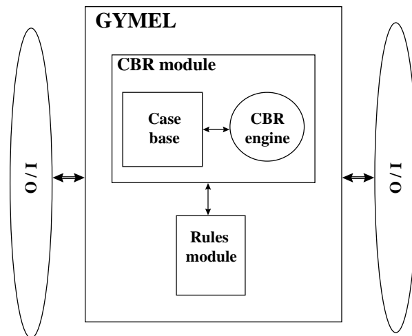
Figure 1. General structure of GYMEL.
