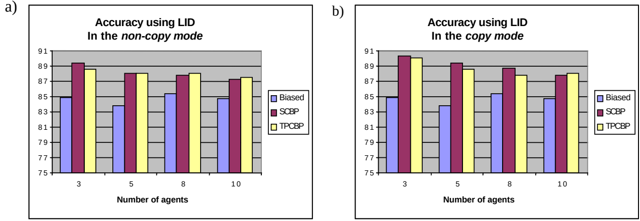
Figure 5: Accuracy plot for systems where the agents use LID
