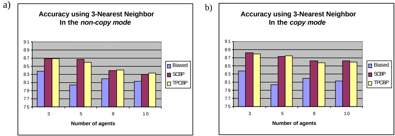
Figure 4: Accuracy plot for systems where the agents use 3-nearest neighbor
