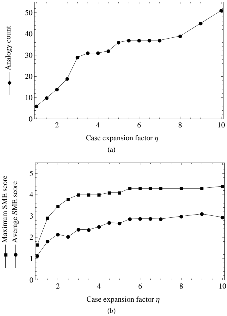
Figure 100: Plots of (a) the number of analogies and (b) the maximum and average SME structural evaluation scores, corresponding to a given case expansion factor \eta . Computations are performed for the Orange case.
