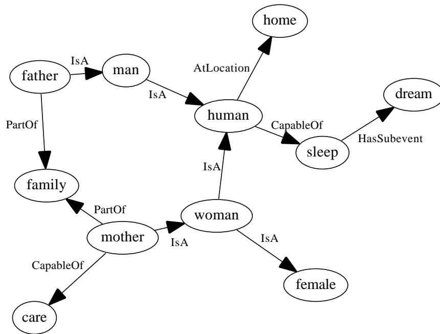
Figure 58: Experiment 2: Given semantic network, 11 concepts, 11 relations (base domain).
