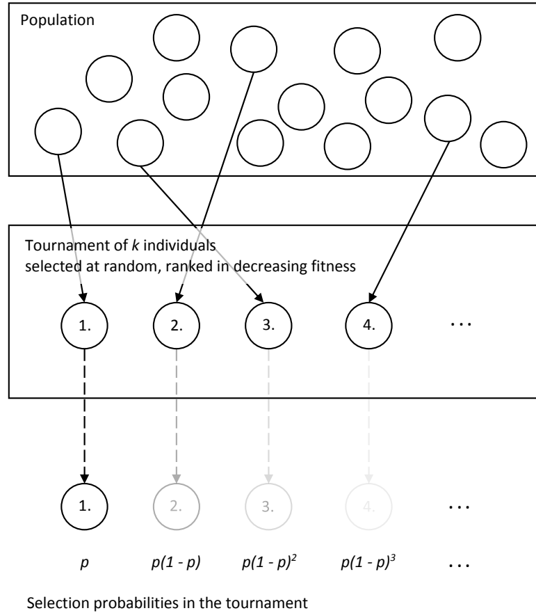
Figure 35: The tournament selection process.
