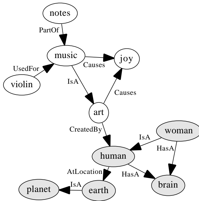
Figure 42: Commonsense crossover type II (graph merging crossover). Offspring, merging by the relation CreatedBy(art, human) . If no concepts attachable through commonsense relations are encountered, the offspring is formed by merging the parent networks as two separate clusters within the same semantic network.
