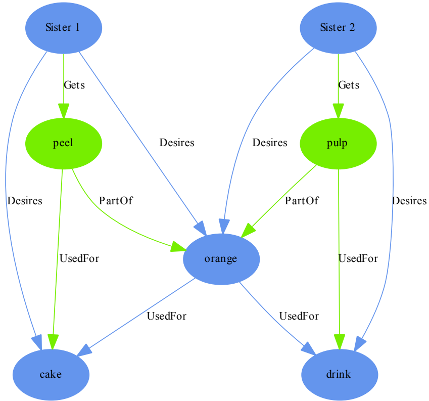
Figure 67: The orange dispute case, fused representation of solved and unsolved case networks. Blue (or dark) color represents the unsolved network, green (or light) color represents the additions/-modifications for solution.
