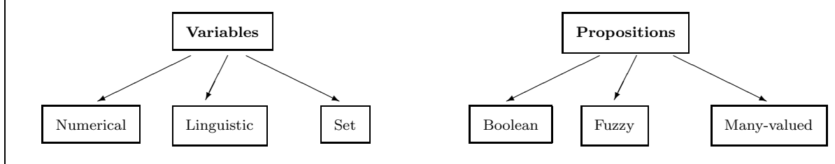
Fig. 2. Types of variables and propositions.
