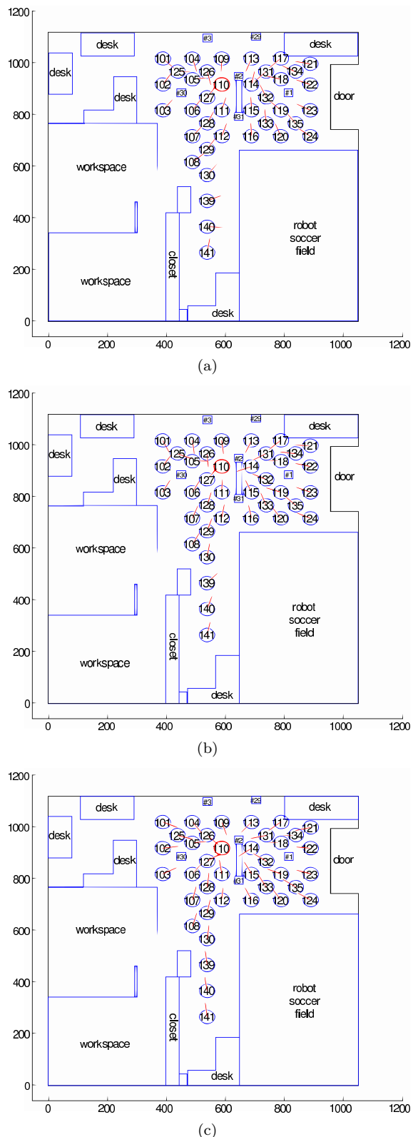
Fig. 8 Homing to panorama 110 in the robotics laboratory using DoG feature points (a), MSER feature points (b) and landmarks (c). All measures are in cm.
