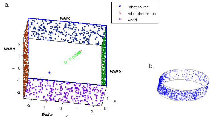
Fig. 6 a) The simulated environment with uniformly randomly spread feature points. b) Panoramic projection of the world used as input for the robot homing system.
