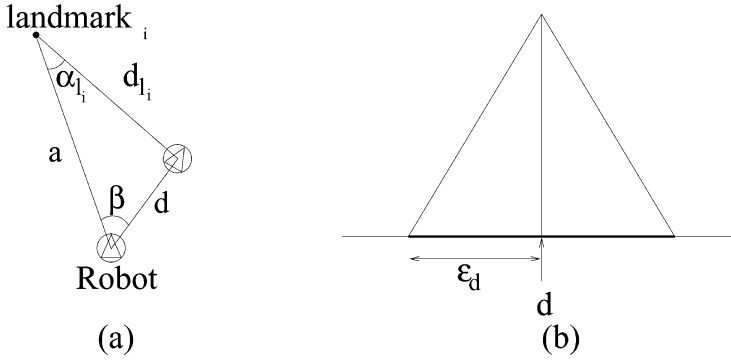
FIGURE 5 (a) Robot movement and angle variation and (b) Fuzzy distance and error
