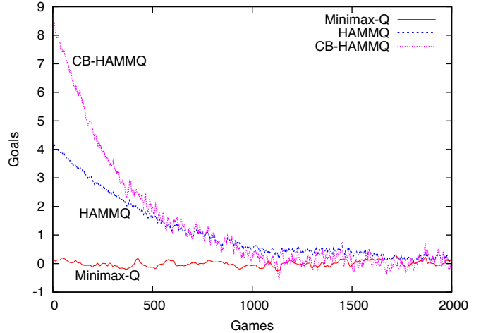
Figure 3. Goals balance for Minimax-Q, the HAMMQ and the CB-HAMMQ algorithms against an opponent using Minimax-Q for the Expanded Littman’s Robotic Soccer.
