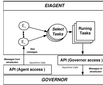
Fig. 3. EIAgent's abstract architecture
