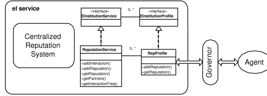
Fig. 2. Centralized reputation system as an eI service
