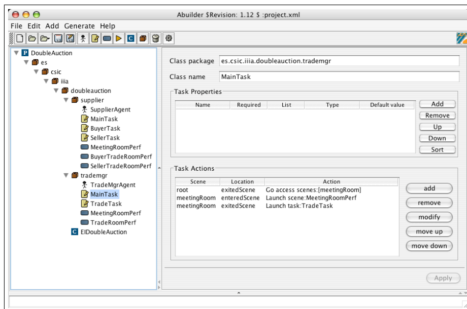
FIGURE 5. aBUILDER GUI
