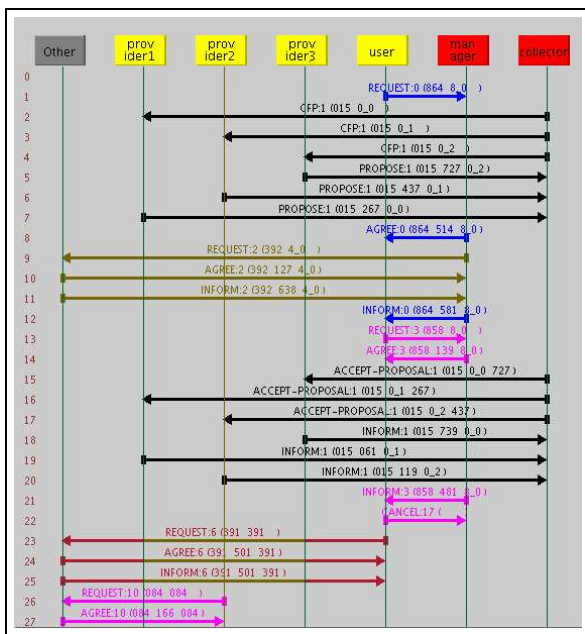
Figure 2. Interaction protocol among trading agents and the iBundler agency
