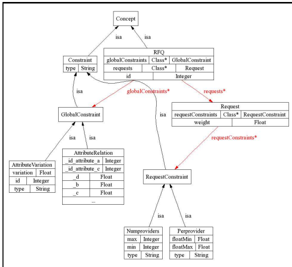
Figure 3. RFQ concept representation
