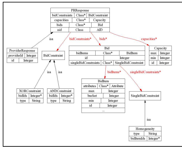
Figure 4. Bid representation as part of the provider response concept
