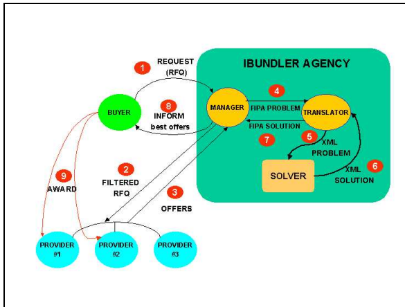
Figure 1. Architecture of the iBundler agency
