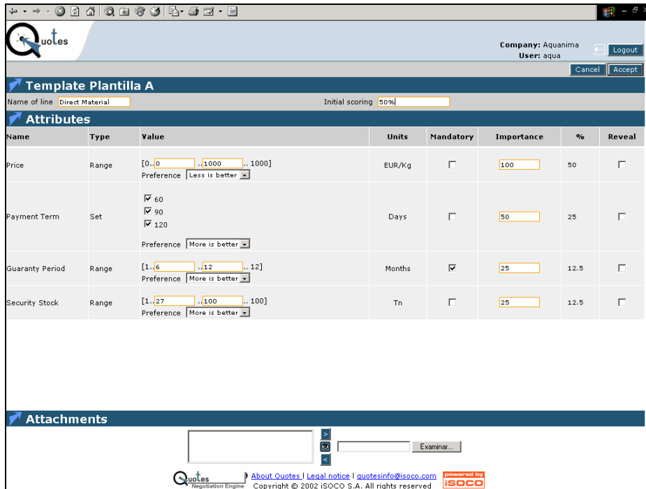
Figure 1: RFQ item creation interface
