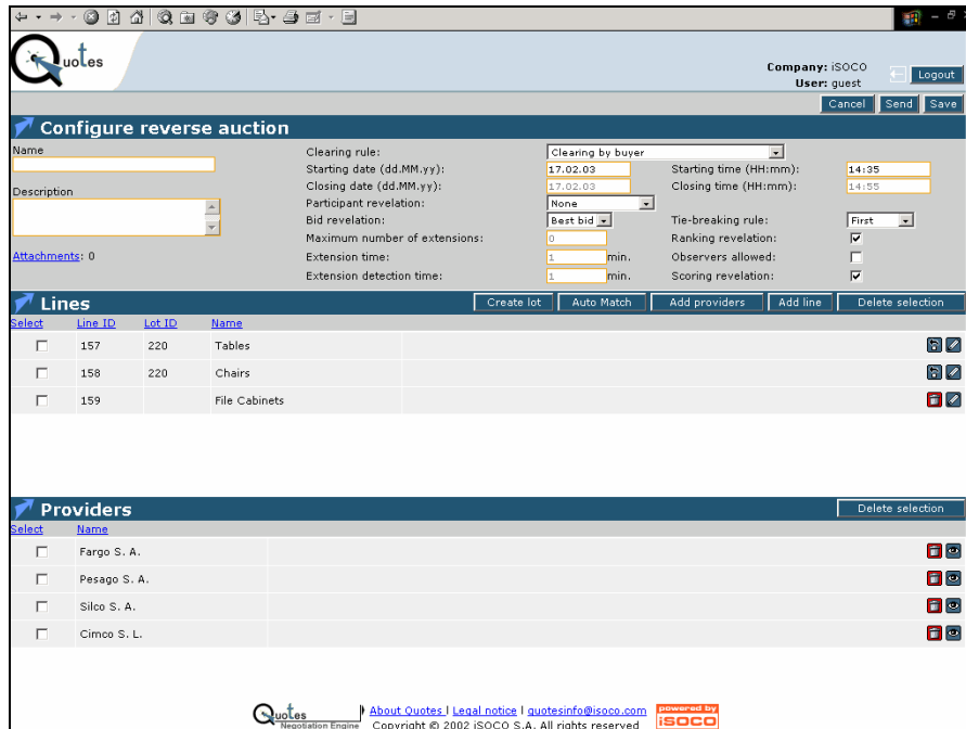
Figure 3. RFQ configuration as a Reverse Auction
