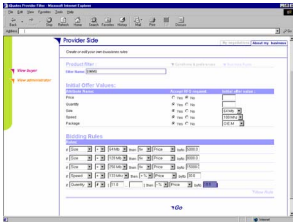
Figure 5: Bidding rule examples
