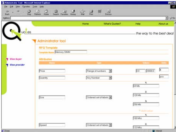
Figure 2: A product template definition
