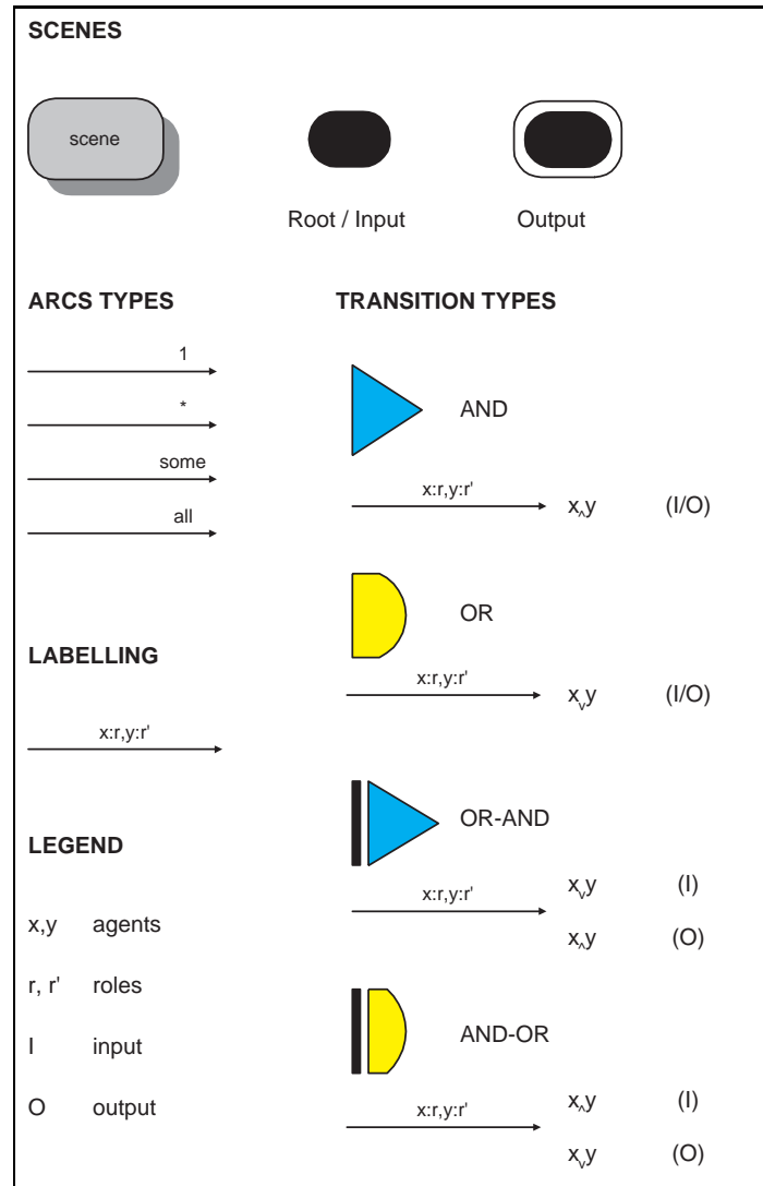
Fig. 2. Graphical Elements of a Performative Structure
