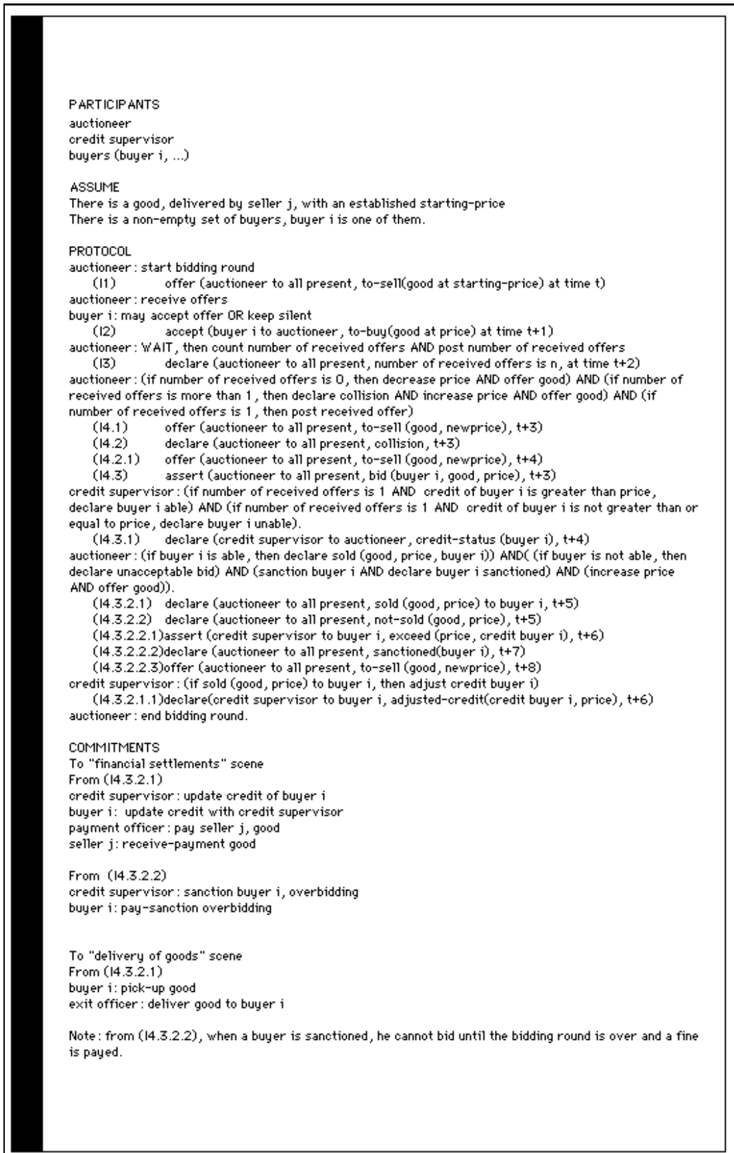
Figure 2: The Fishmarket downward bidding protocol. Naive communication flow.
