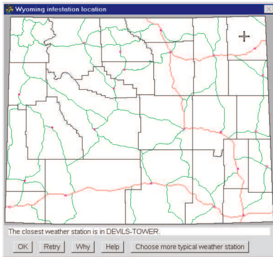
Figure 4: CARMA's interface window for determining infestation location.
