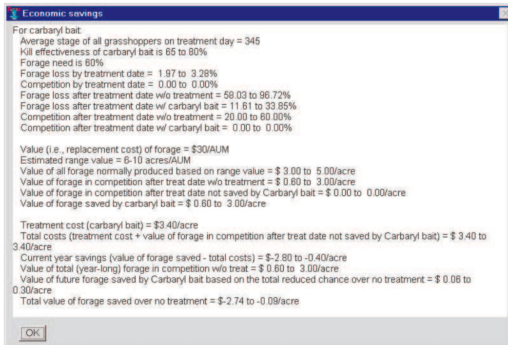
Figure 11: Interface window explaining CARMA's economic savings calculations.
