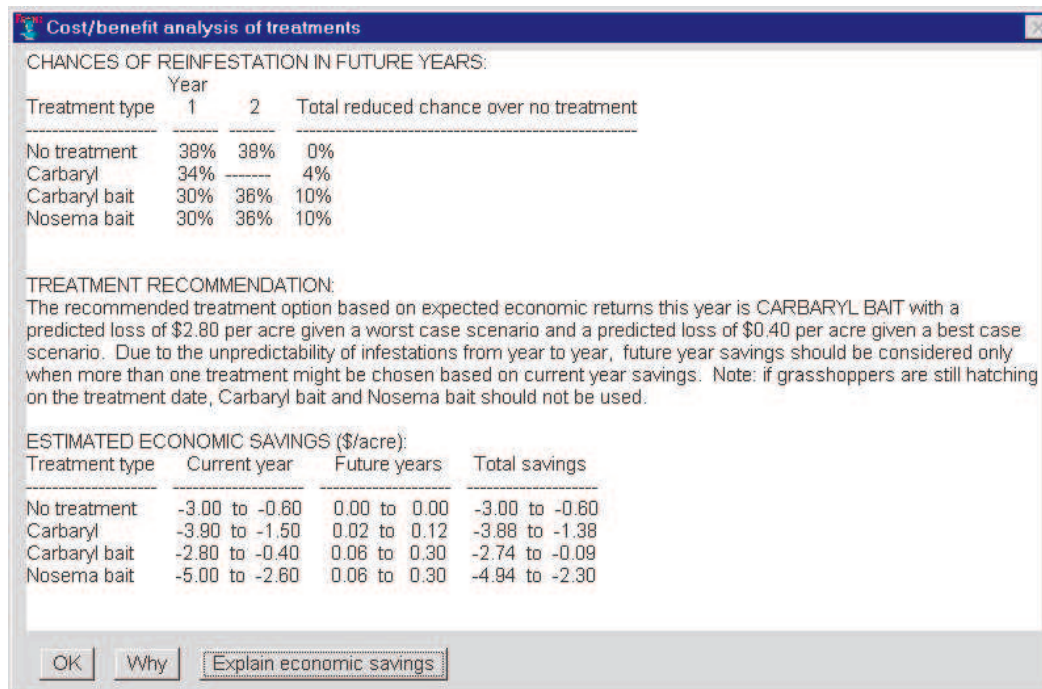
Figure 10: CARMA's interface window recommending a treatment option and estimating the probability of future reinfestation and economic savings. The dashed line in the second-year reinfestation probability for carbaryl indicates no reduction in infestation probability for that year.
