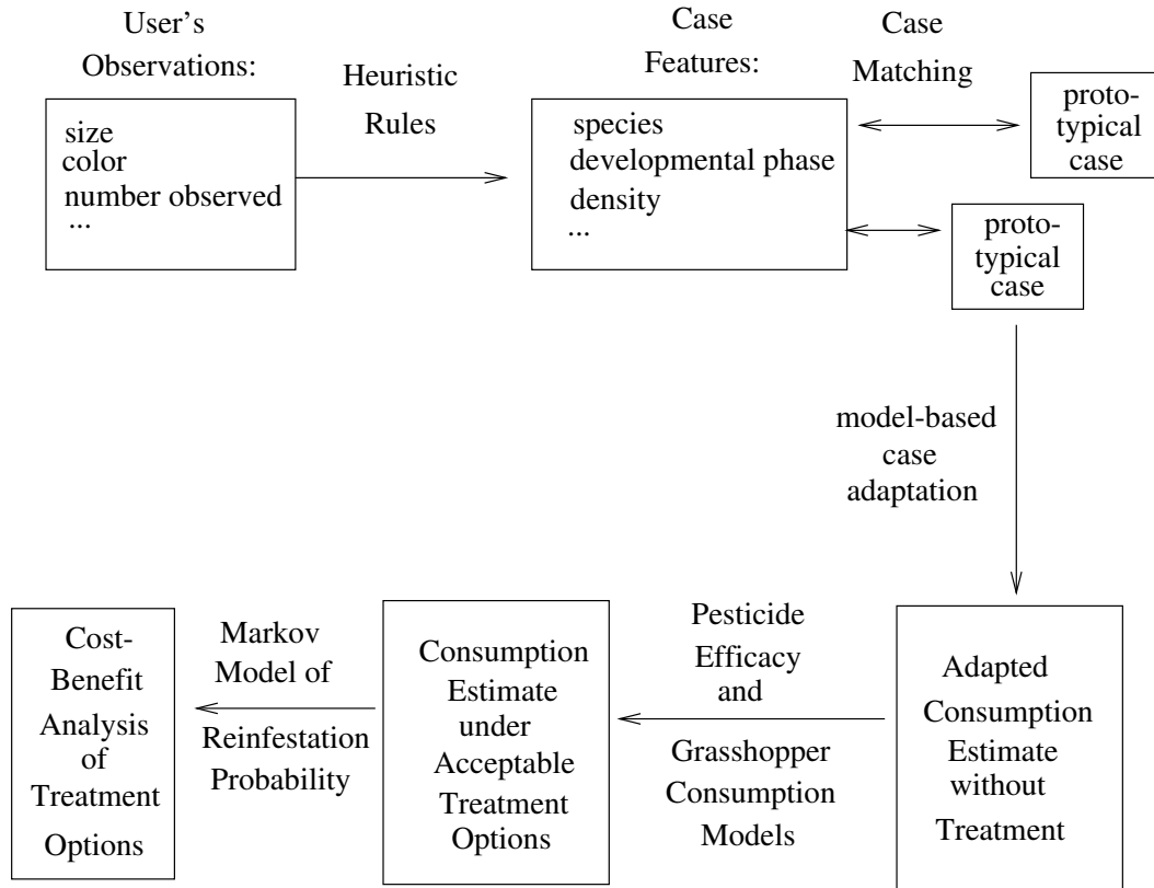
Figure 2: The main steps in CARMA's consultation process.
