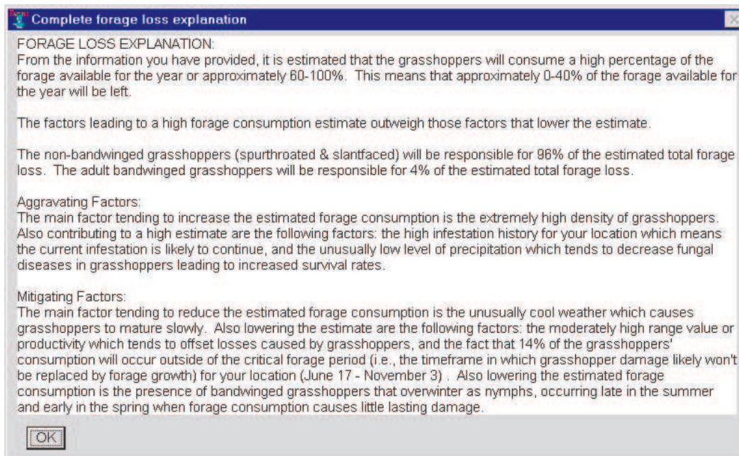
Figure 7: Interface window explaining CARMA's estimate of forage loss.
