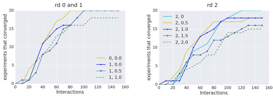
Figure 2. Results for a vocabulary of 4 words and protocols with 8 common constraints
