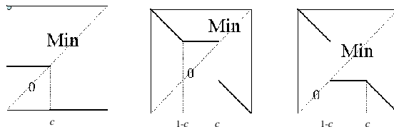
Figure 1: WNM t-norms *_c , \star_c and \circ_c , respectively.
